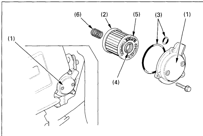
Fig. 4-13 (1) Oil filter cover (2) Oil filter (3) O-rings
