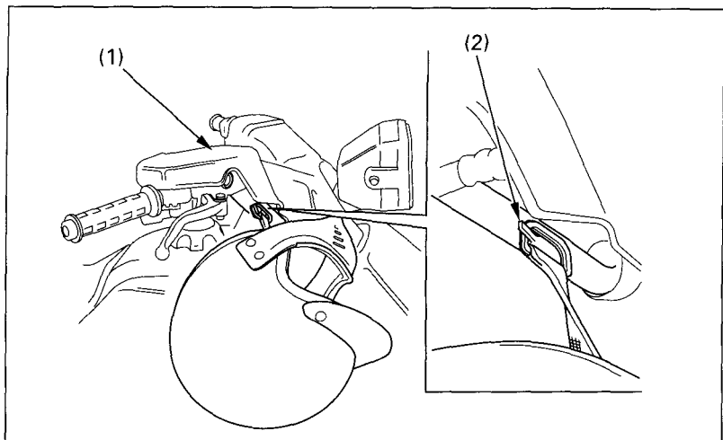
Fig. 2-22 (1) Handlebar cover
