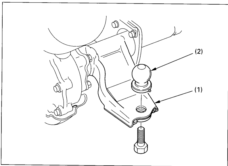
Fig. 2-25 (1) Trailer hitch
