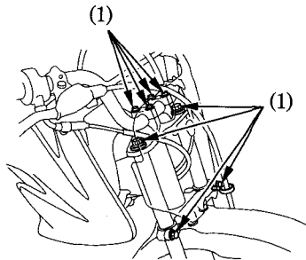
(1) Mounting bolts
